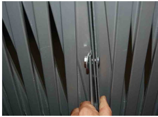
Step 8. Attach the denter strut and add bolts to the top and bottom of the gate sections.
