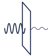
SOUND DAMPENING
